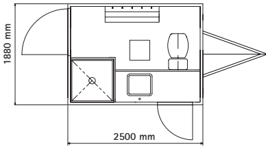
Model 250 - bad/toilet
